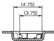
SECT E-E
